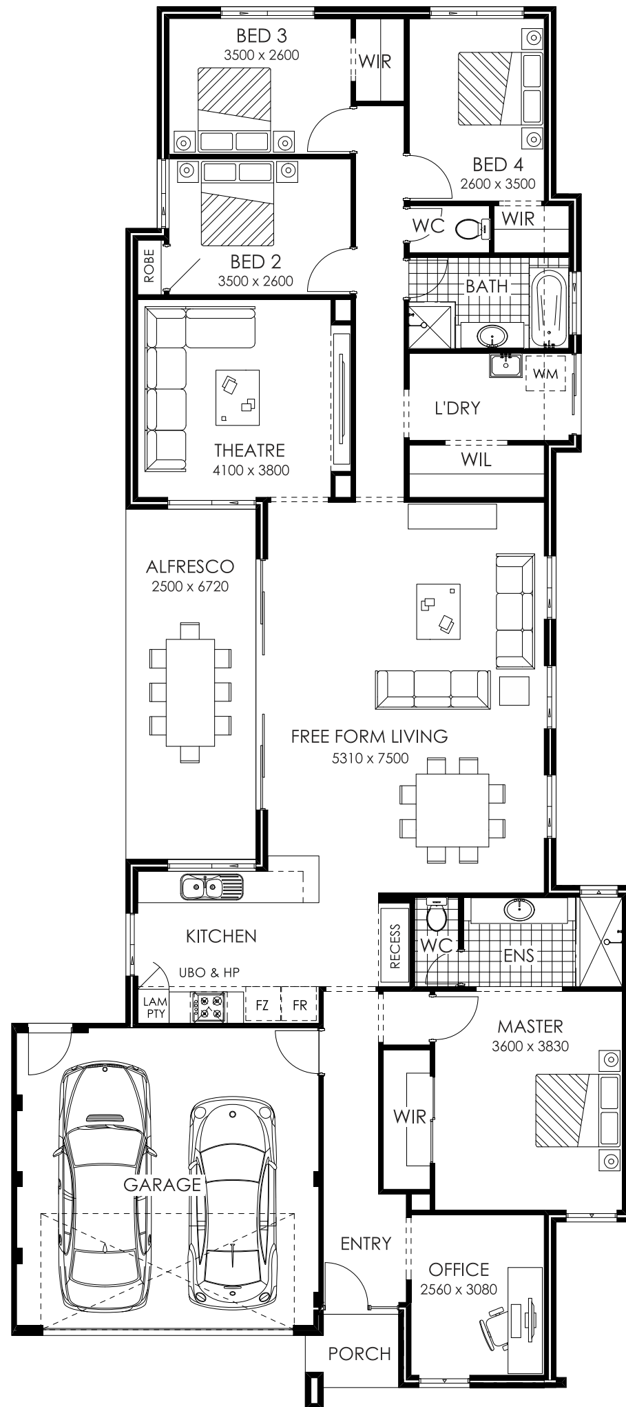
GROUND FLOOR
